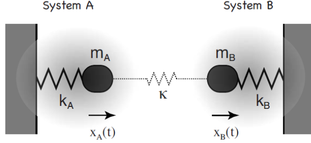
Figure 2.5: Analog of light-matter interaction: two mechanical oscillators (masses m_A , m_B , spring constants k_A , k_B ) coupled by a spring \kappa . [39].
