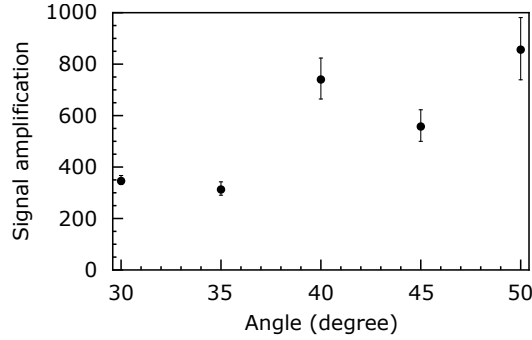
Figure 4.9: Angular dependence of the signal amplification. The probe beam fluence is kept at \sim 20 \text{ nJ cm}^{-2} while the pump power is fixed at 180 \text{ } \mu\text{J cm}^{-2}
