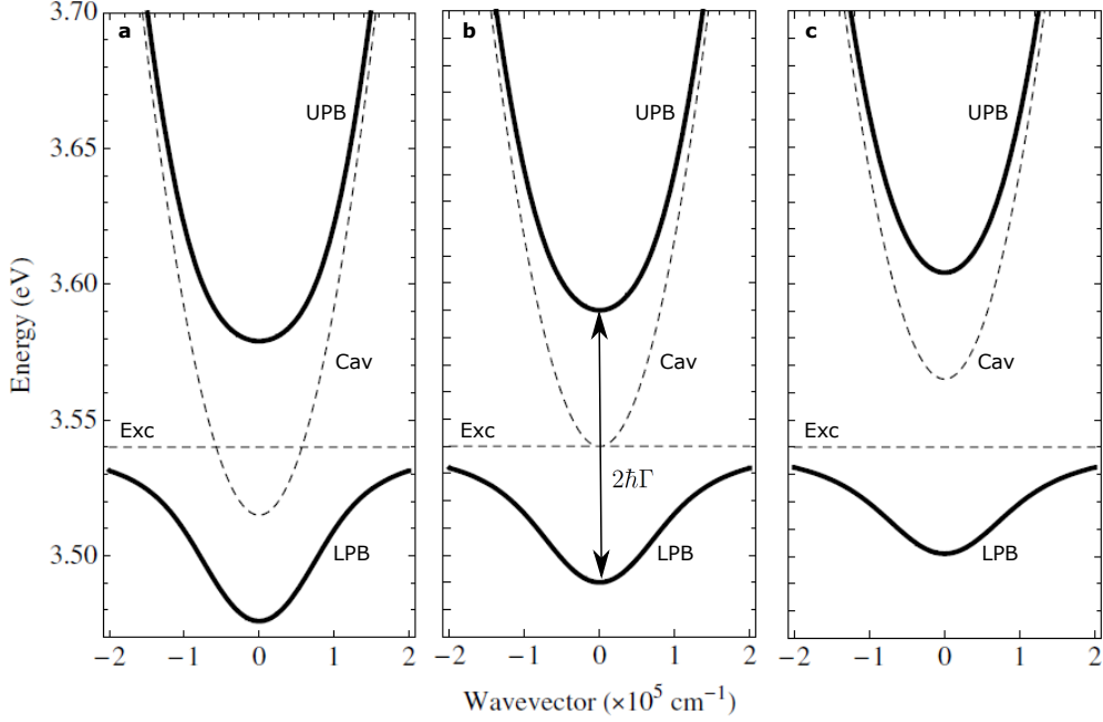
Figure 2.6: Illustration of the strong exciton-photon coupling for three values of detuning. Adapted from [33].
