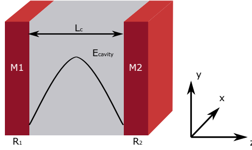
Figure 2.1: The schematic of an optical microcavity. Light is confined between the mirrors M1 and M2 having the separation distance of \frac{\lambda_c}{2n_c} .
