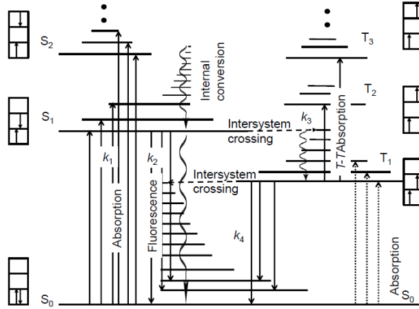
Figure 2.3: A typical Jablonski diagram depicting molecular energy states together with possible transitions [37].
