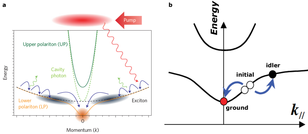
Figure 2.7: Polariton lasing buildup in inorganic microcavities. (a) A relaxation route towards the ground polariton state under nonresonant pumping. Taken from [20]. (b) A schematic of polariton-polariton scattering [42].
