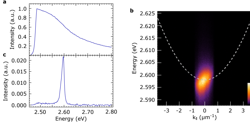
Figure 4.2: Seeding the ground polariton state. (a) The spectrum of the broadband probe before the sample. (b) Energy and momentum resolve emission image obtained with the seeding by the probe. The white dashed line is a fit for LPB below the threshold (c) The spectrum of the probe after the sample.
