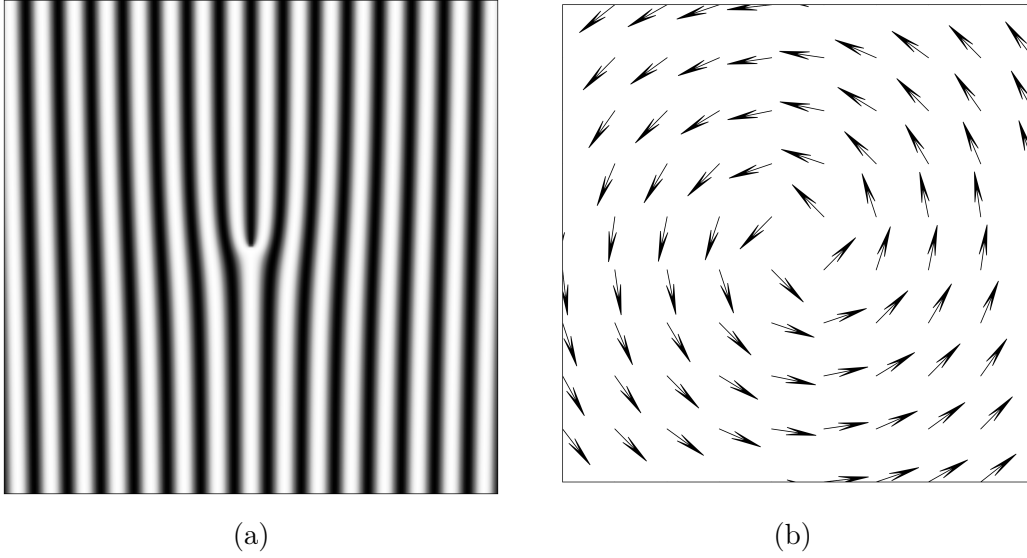
Figure 4-9: Mapping of the topological defects of the CDW to the DGPE lattice: (a) a dislocation of the CDW order, u(\mathbf{r}) \exp(i\phi(\mathbf{r})) , plotted as a 2D map of the electronic density modulation defined by Eq. (4.1)—white and black represent the CDW regions with the increased and decreased electronic density respectively, (b) a vortex of the DGPE lattice corresponding to the CDW dislocation after the mapping—each arrow represents \psi_j .
