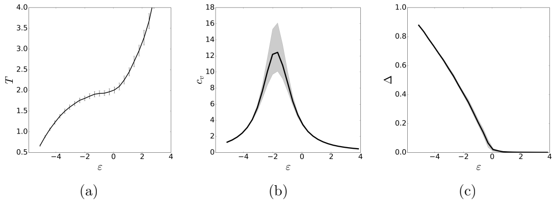
Figure 4-4: Signatures of the spontaneous symmetry breaking in the 3D DGPE lattice: (a) temperature, T(\varepsilon) , (b) specific heat c_v(\varepsilon) and (c) the order parameter, \Delta(\varepsilon) as functions of the energy density \varepsilon .
