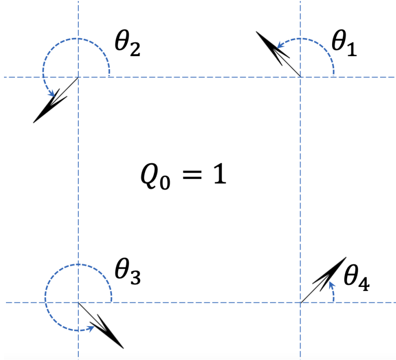
Figure 4-7: Example of a DGPE plaquette with vorticity Q_0 = 1 according to Eq. (4.30).
