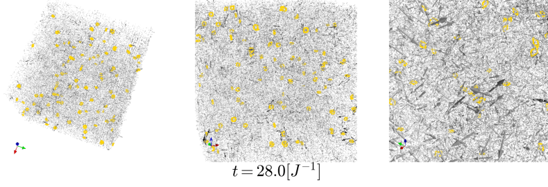
(a) Snapshot for the blue dot in Fig. 4-10
