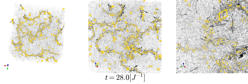
(c) Snapshot for the red dot in Fig. 4-10
