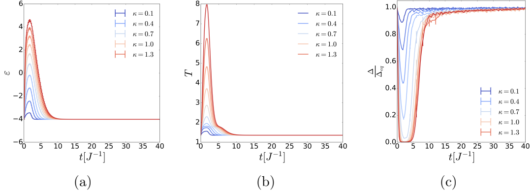
Figure 4-5: The non-equilibrium quench protocol. (a) energy density, \varepsilon(t) , (b) temperature, T(t) , (c) the order parameter normalized to its equilibrium value \Delta(t)/\Delta_{eq} — all as a function of time after the quench. Color represents the value of the quenching rate \kappa .
