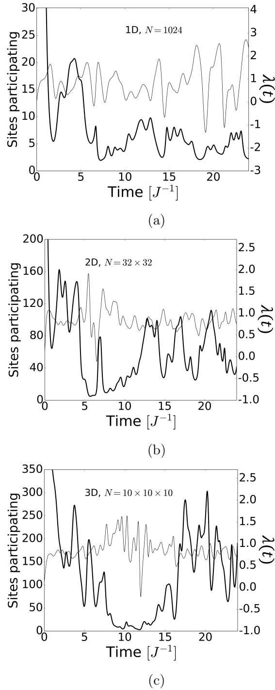
Figure 3-1: Fluctuations of instantaneous stretching rates \lambda(t) (thin black lines) and the number of sites participating in the Lyapunov eigenvector (thick black lines) for: (a) a 1D chain of 1024 sites, (b) a 2D square lattice 32 \times 32 , (c) a 3D cubic lattice 10 \times 10 \times 10 .
