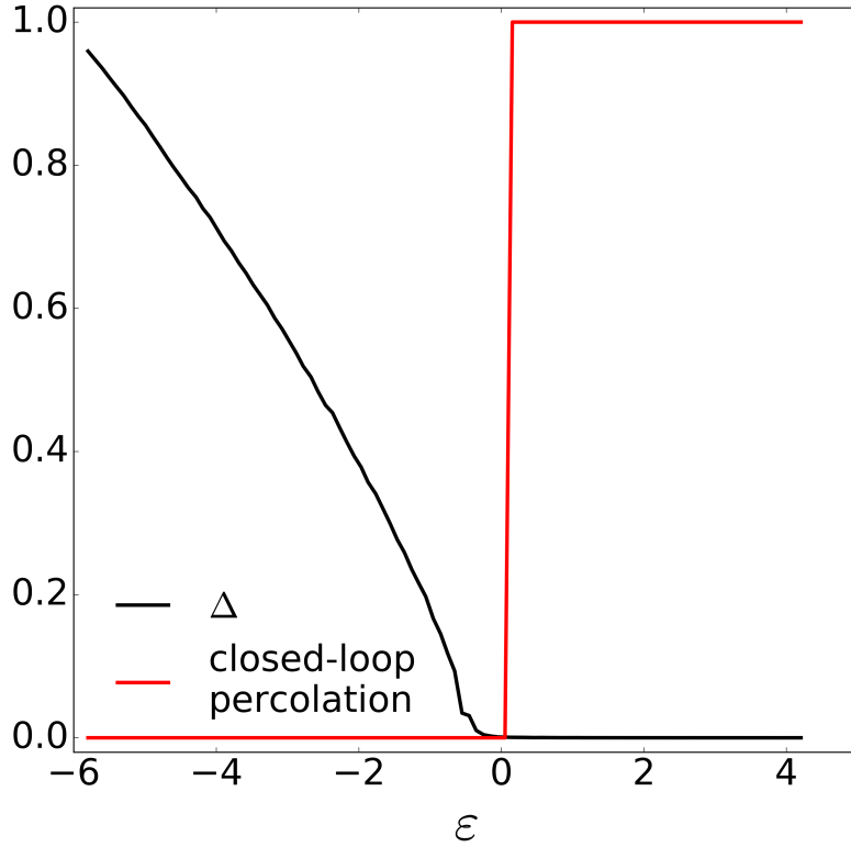
Figure 4-8: A non-contractible loop percolation as the reason for the symmetry breaking in the 3D DGPE lattice. Black line—the order parameter, \Delta(\varepsilon) , as functions of the energy density, red line—the presence of a non-contractible closed-loop vortex in the system (0—no such loop, 1—the loop has percolated). The system's volume V = 30^3 .
