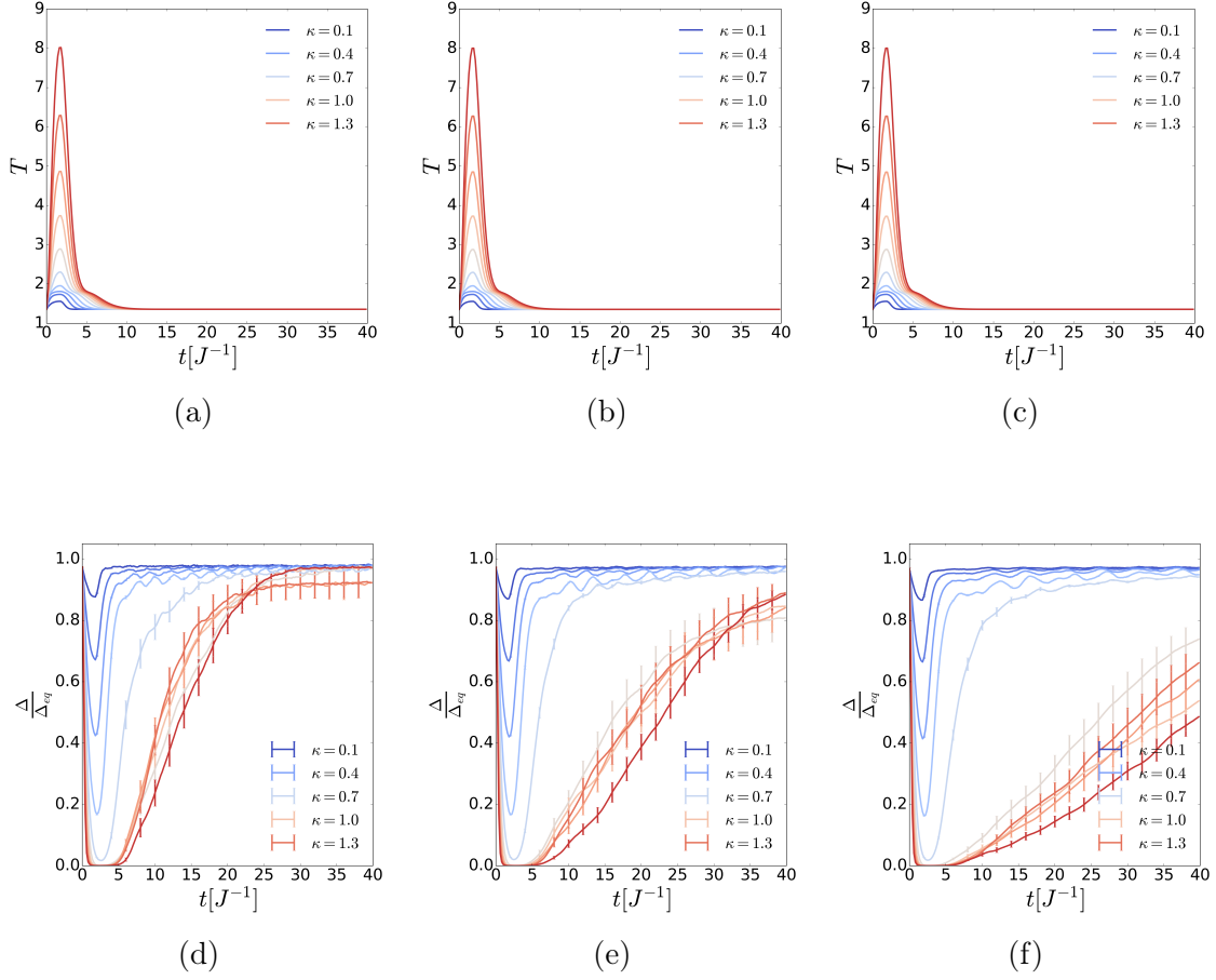
Figure 4-6: System size scaling of the order parameter recovery after the quench: \Delta(t)/\Delta_{eq} for almost identical quenching protocol T(t) . Upper panel: T(t) . Lower panel: \Delta(t)/\Delta_{eq} . The system sizes: (a,d) V = 20^3 , (b,e) V = 30^3 , (c,f) V = 40^3 . Color represents the value of the quenching rate \kappa .
