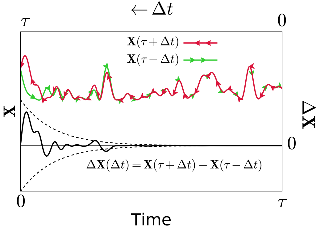
Figure 1-1: Sketch of a slightly imperfect noise reversal. Equilibrium noise of an observable \mathbf{X} before and after an imperfect time reversal of a system's dynamics at time \tau is denoted, respectively, as \mathbf{X}(\tau - \Delta t) (green line) and \mathbf{X}(\tau + \Delta t) (red line), where \Delta t = |\tau - t| . In order to facilitate visual comparison, “Time” on the horizontal axis represents t before the time reversal and 2\tau - t after the time reversal. The difference between the direct and the reversed noise \Delta \mathbf{X}(\Delta t) \equiv \mathbf{X}(\tau + \Delta t) - \mathbf{X}(\tau - \Delta t) (thick black line) fluctuates around 0. For a chaotic system, the envelope of \Delta \mathbf{X}(\Delta t) grows exponentially (dashed lines).
