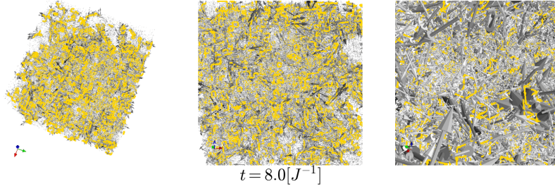
(a) Snapshot at time t = 8[J^{-1}]
