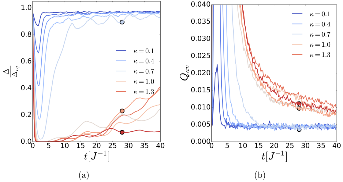
Figure 4-10: Illustration of the role of topological defects in the slowing down of the order parameter recovery for V = 50^3 : (a) order parameter normalized to its equilibrium value \Delta(t)/\Delta_{eq} as a function of time; (b) the average vorticity Q_{av}(t) for the same system. Color represents the value of the quenching control parameter \kappa as indicated in the plot legend. The states corresponding to the three points (red, pink, blue) in each of the plots are to be analyzed below in more detail.
