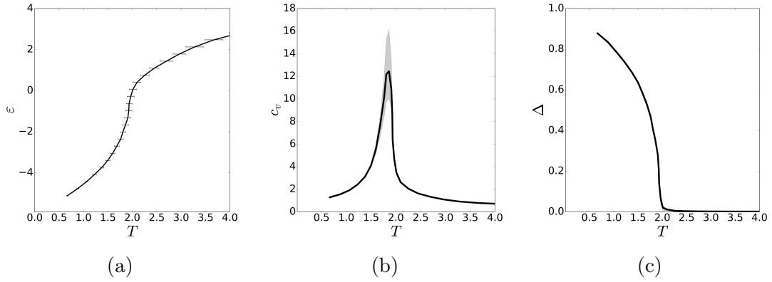
Figure 4-3: Signatures of the spontaneous symmetry breaking in the 3D DGPE lattice: (a) energy density, \varepsilon(T) , (b) specific heat c_v(T) and (c) the order parameter, \Delta(T) as functions of temperature T .
