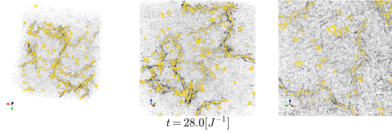
(b) Snapshot for the pink dot in Fig. 4-10
