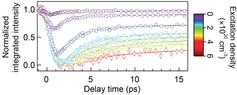
Figure 4-1: Time evolution of integrated intensity of the CDW electron diffraction peak after photo-excitation at varying laser pulse intensities (photo-excitation densities). The figure reproduced from Ref. [230] in adapted form.
