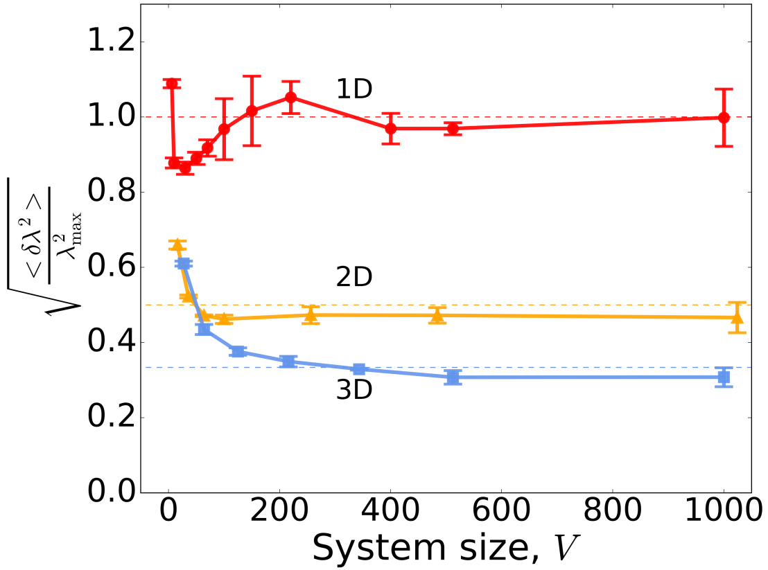
Figure 3-3: Numerical test of empirical estimate (3.21) for \langle \delta \lambda^2 \rangle . The dependence of \sqrt{\langle \delta \lambda^2 \rangle / \lambda_{\max}^2} on the number of lattice sites V for one- (red circles), two- (orange triangles) and three-dimensional (light blue squares) lattices. The dashed lines are plotted at the levels of 1/d , where d is the lattice dimension.
