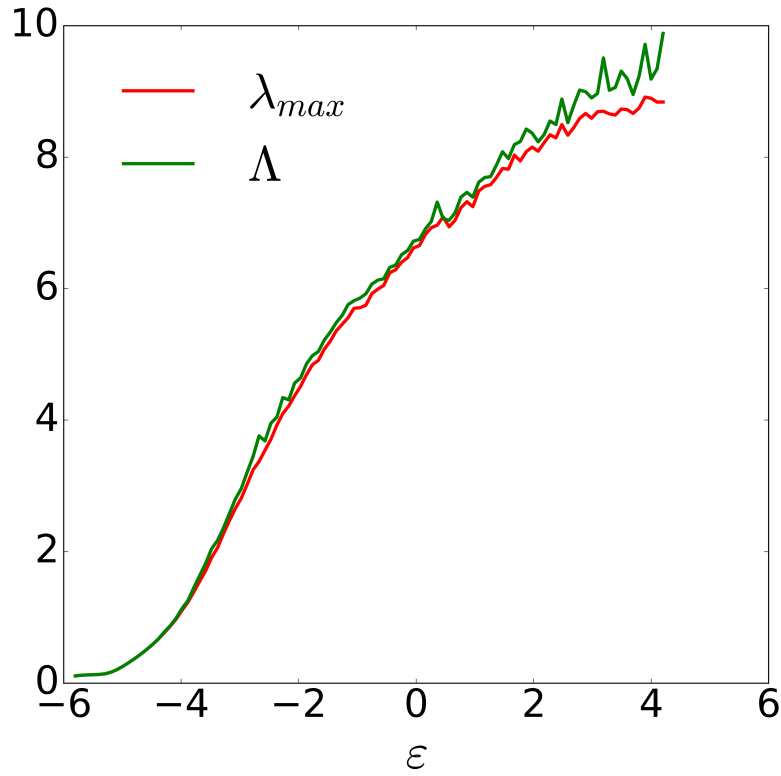
Figure 4-14: Estimating the ergodization time of the 3D DGPE lattice for the energy range containing a spontaneous symmetry breaking. The results of Loschmidt echoes simulations: (red line) the largest Lyapunov exponent \lambda_{max} from Eq. (2.2), and (green line) \Lambda from Eq. (3.3) as functions of the energy density, \varepsilon . The difference \Lambda - \lambda_{max} is proportional to the ergodization time according to Eq. (3.22).
