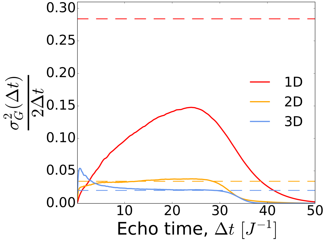
Figure 3-5: Ergodicity tests. The dependence of the ratio \frac{\sigma_G^2(\Delta t)}{2\Delta t} on the echo time \Delta t for a 1D chain of 100 sites (red), a 2D square lattice 10 \times 10 (orange), a 3D cubic lattice 4 \times 4 \times 4 (light blue). The dashed lines are plotted at the levels \Lambda - \lambda_{\max} corresponding to the plateaux expected for ergodizing systems. These plots imply that the 2D and 3D lattices are ergodized on the timescale of the simulations, while the 1D lattice is not.
