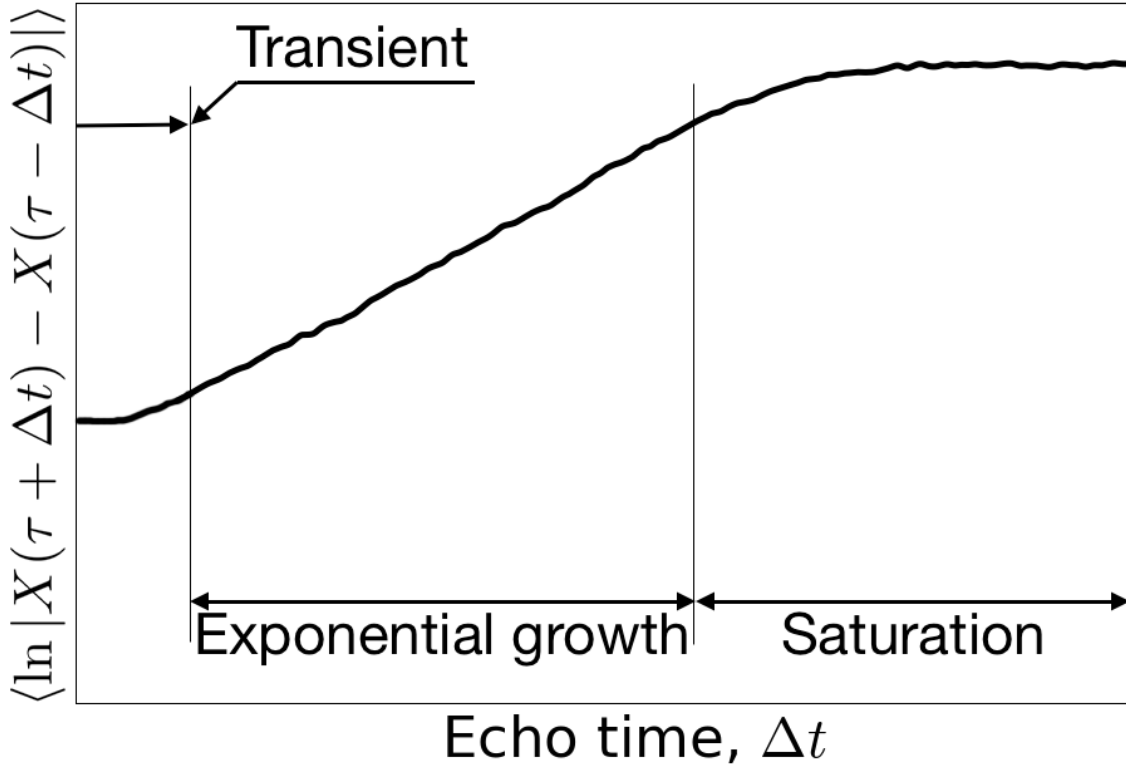
Figure 2-1: Sketch of a typical Loschmidt echo response \langle \log |X(\tau + \Delta t) - X(\tau - \Delta t)| \rangle (thick black line). Three characteristic regimes described in the text are indicated: transient, exponential growth and saturation.
