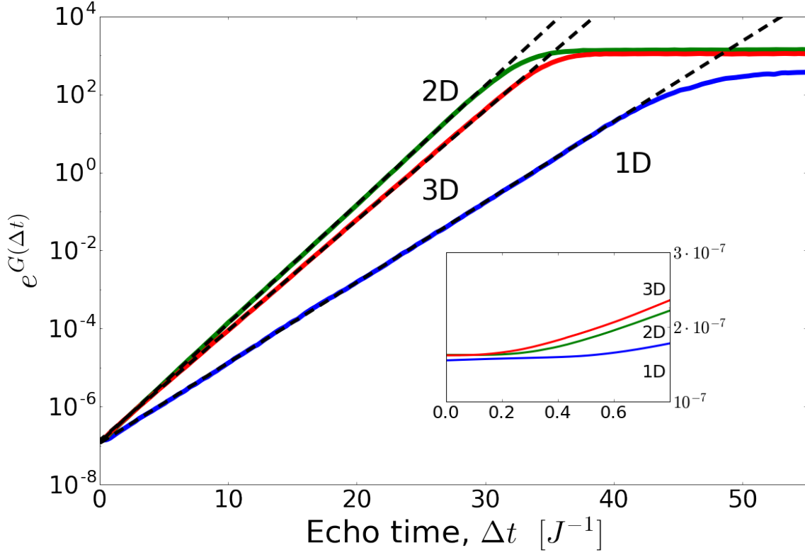
Figure 2-3: Loschmidt echo response \exp(G(\Delta t)) obtained from Eq. (2.2) for a one-dimensional chain of 10 sites (1D, blue line), a two-dimensional 10 \times 10 square lattice (2D, green line) and a three-dimensional 4 \times 4 \times 4 cubic lattice (3D, red line). The inset shows the behavior of \exp(G(\Delta t)) in the transient regime at small echo times, where all Lyapunov exponents contribute to the growth. The transient regime takes longer time for lower dimensions. In Table 2.1, the values of \lambda_{\max} obtained by fitting the exponential growth regime according to Eq. (2.2) are compared to the results of averaging of instantaneous stretching rates from Eq. (2.3).
