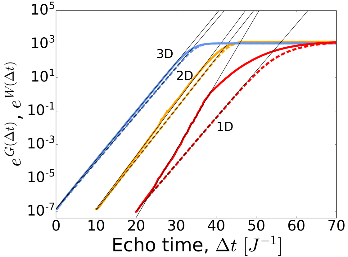
Figure 3-4: Loschmidt echo responses G(\Delta t) defined according to Eq. (2.2) (dashed lines), and W(\Delta t) defined by Eq. (3.3) (solid lines) for: a three-dimensional 4 \times 4 \times 4 cubic lattice (3D, light blue); a two-dimensional 10 \times 10 square lattice (2D, orange, shifted to the right by 10); a one-dimensional chain with 100 sites (1D, red, shifted to the right by 20). Thin black lines are linear fits from which \lambda_{\max} and \Lambda , listed in Table 3.1, were extracted.
