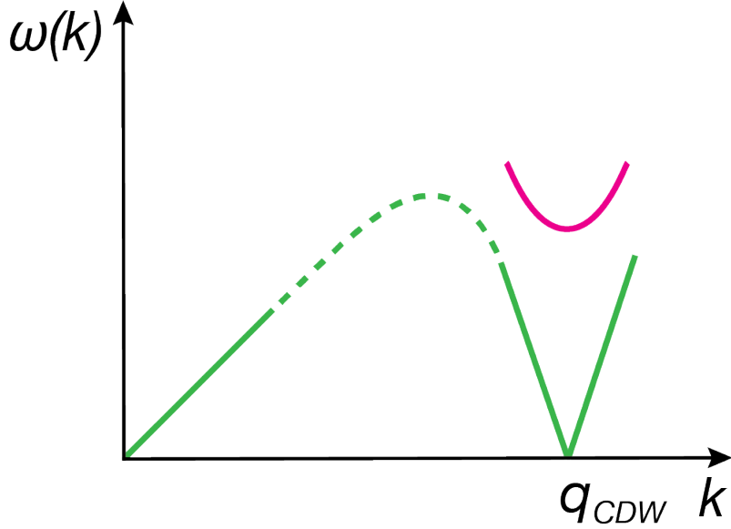
Figure 4-2: A typical acoustic phonon dispersion relation \omega(k) — green line. The acoustic phonon softening associated with the emergence of the CDW is shown as a sharp dip at the CDW wavevector \mathbf{q}_{CDW} . The red line represents the dispersion relation for temperatures higher than the critical temperature. The green dashed line represents the region, where the acoustic phonon modes are ill-defined.
