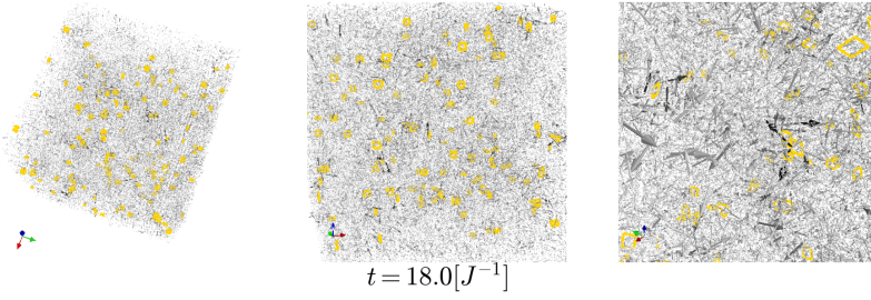
(b) Snapshot at time t = 18[J^{-1}]
