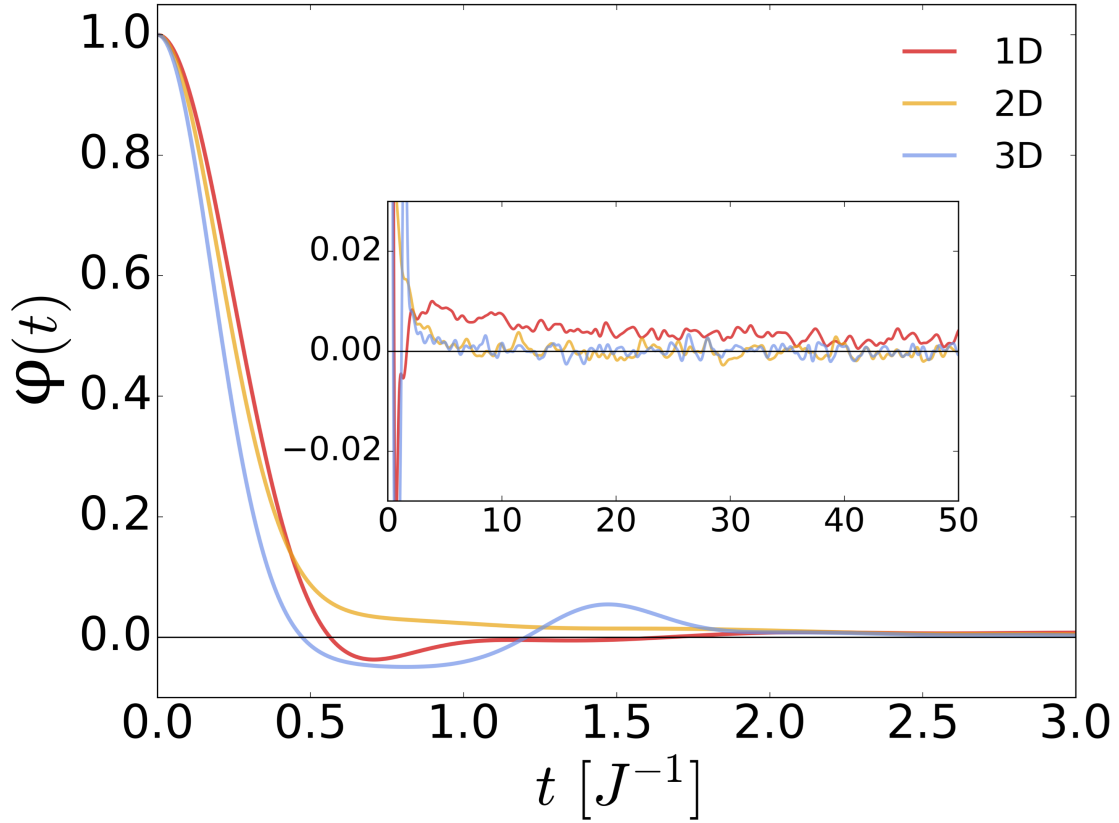
Figure 3-2: Autocorrelation function \varphi(t) for instantaneous stretching rates \lambda(t) for a 1D chain of 100 sites (red), a 2D square lattice 10 \times 10 (orange), a 3D cubic lattice 4 \times 4 \times 4 (light blue). In the inset, the tails of \varphi(t) are plotted for longer times.
