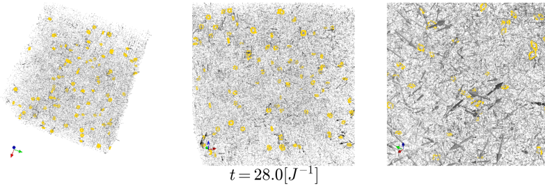
(c) Snapshot at time t = 28[J^{-1}]
