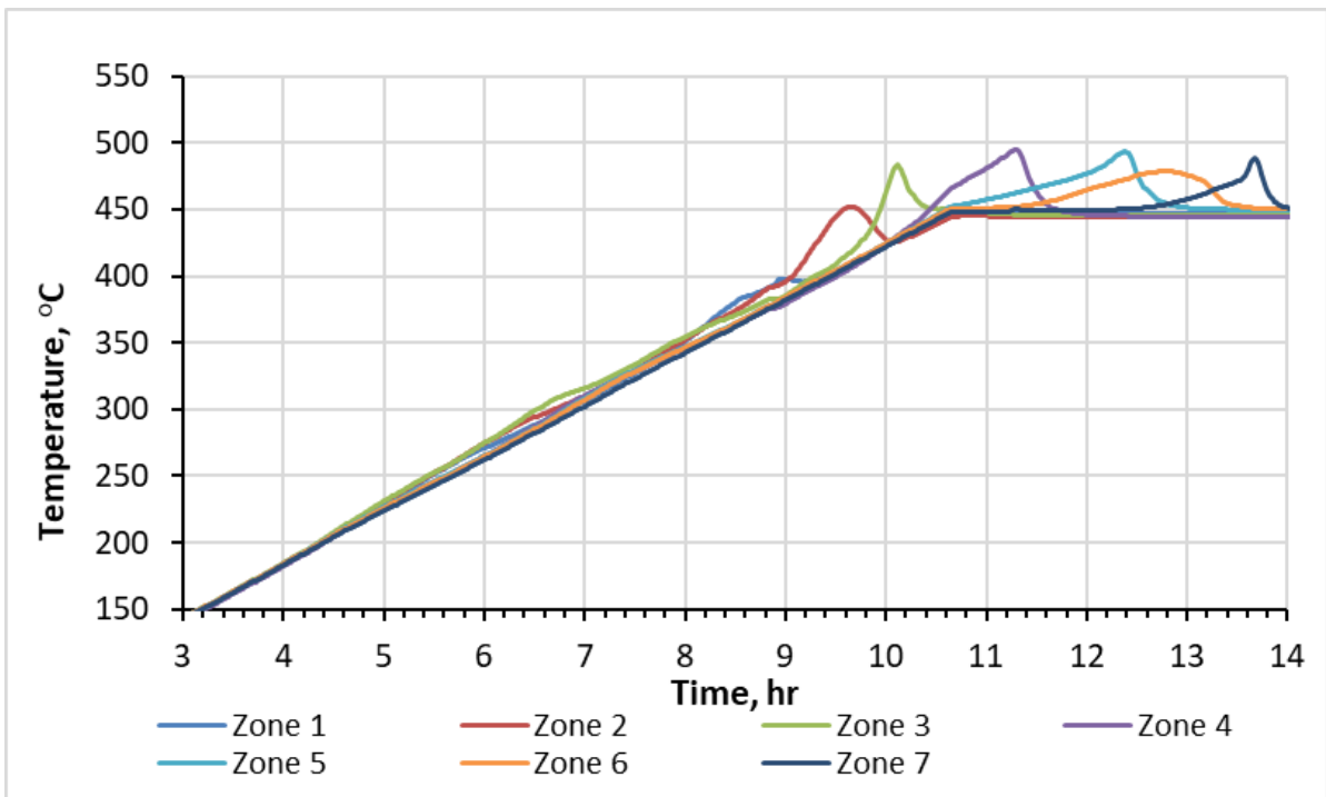
Figure 3.1 Zoom in temperature profiles by zones in the RTO test for bitumen
