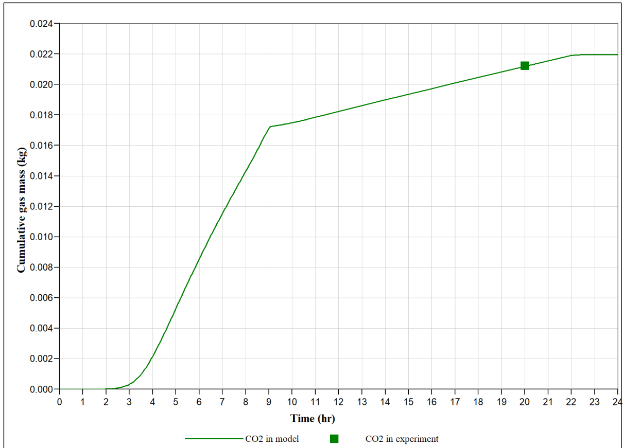
Figure 3.24 Comparison of the results for experiment and simulation for RTO test for carbonate oil example: cumulative gas mass (modified reaction scheme)
