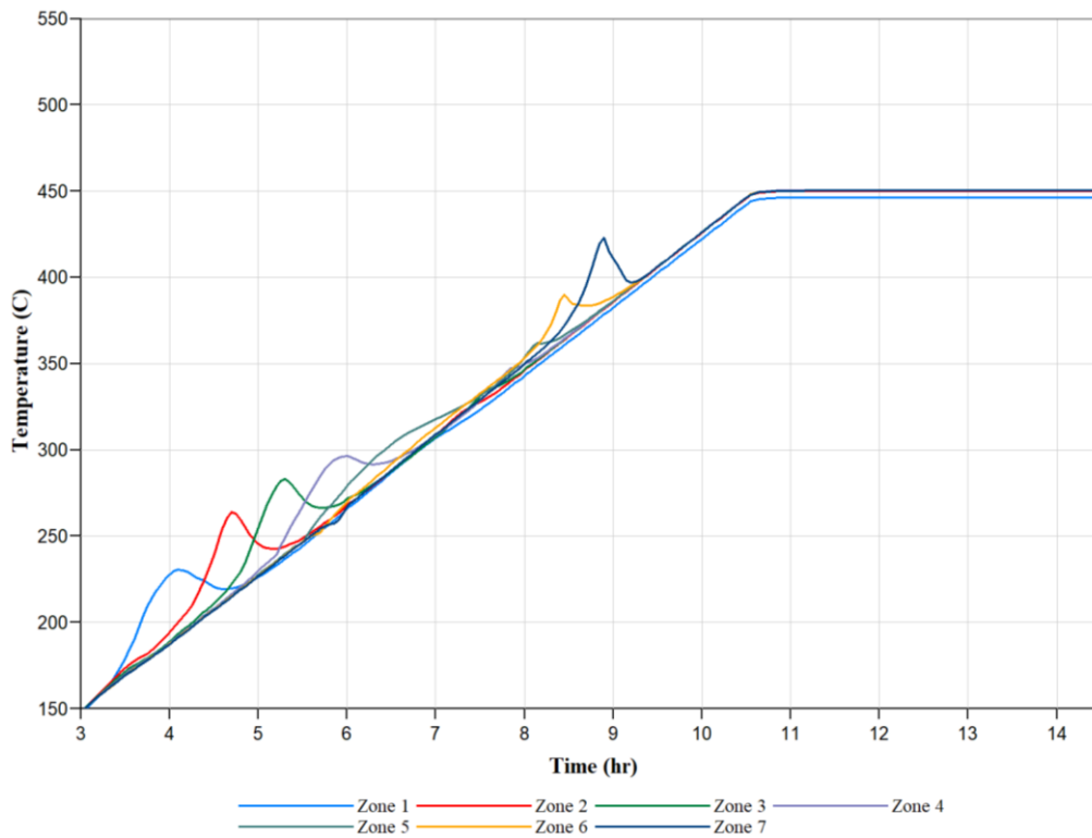
Figure 3.18 Zoom in simulated temperature profiles for the modified reaction model for carbonate oil field
