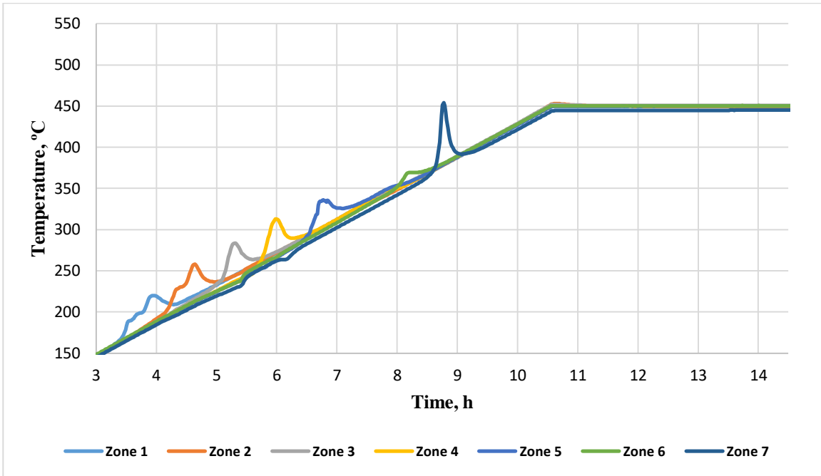
Figure 3.9 Zoom in temperature profiles by zones in RTO test for carbonate oil field
