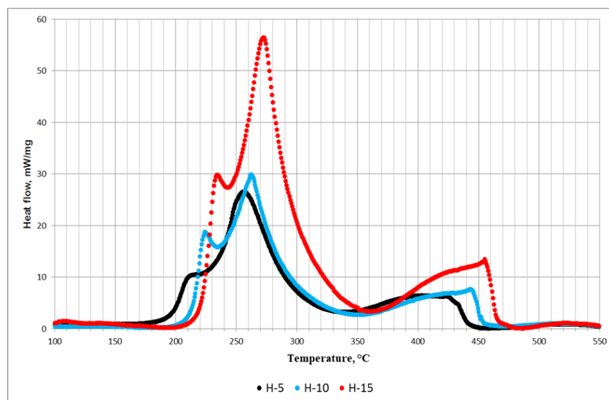
Figure 3.15 Temperature dependence of the heat flow for the original oil sample as a result of PDSC test (black - 5 °C/min, blue – 10 °C/min, red – 15 °C/min)
