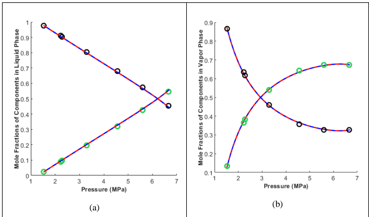
Figure 4.11 Phase compositions at different pressures for the methane—ethane binary mixture at T = 250K
