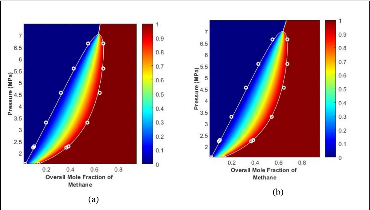
Figure 4.6 Pressure-composition phase diagram for the methane—ethane binary mixture at T = 250\text{K} as a result of a) flash calculations and b) Gibbs minimization algorithm
