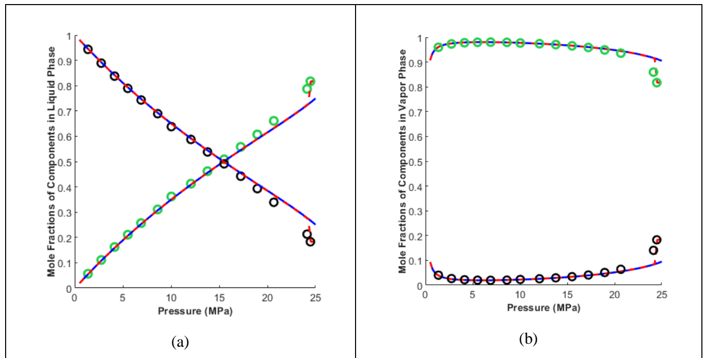
Figure 4.13 Phase compositions at different pressures for the methane—n-heptane binary mixture at T = 344.3 K
