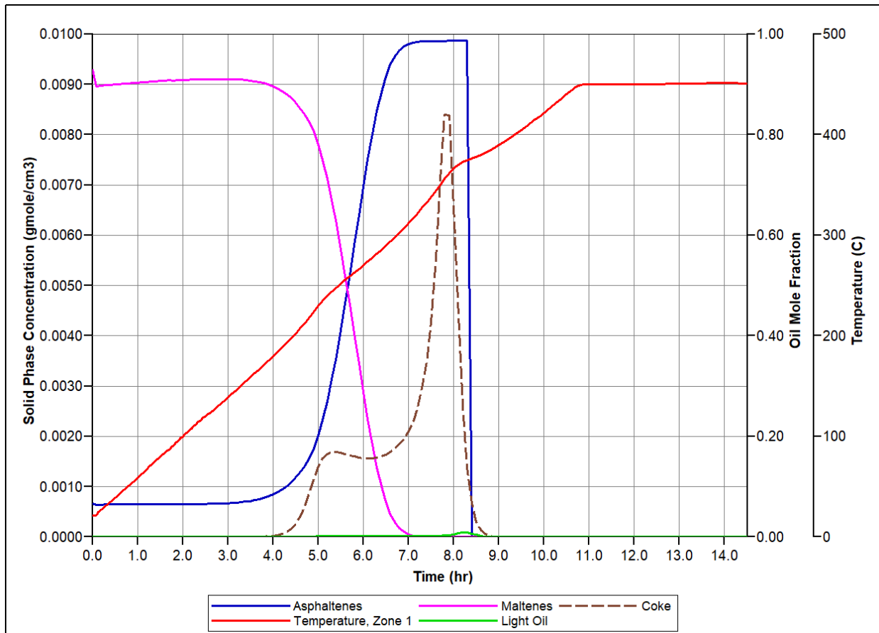
Figure 3.6 Numerical simulation results at 1 Zone of the reactor for RTO test for bitumen: temperature profile, molar fraction of Maltenes, Asphaltenes, Light Oil and solid-phase concentration of Coke
