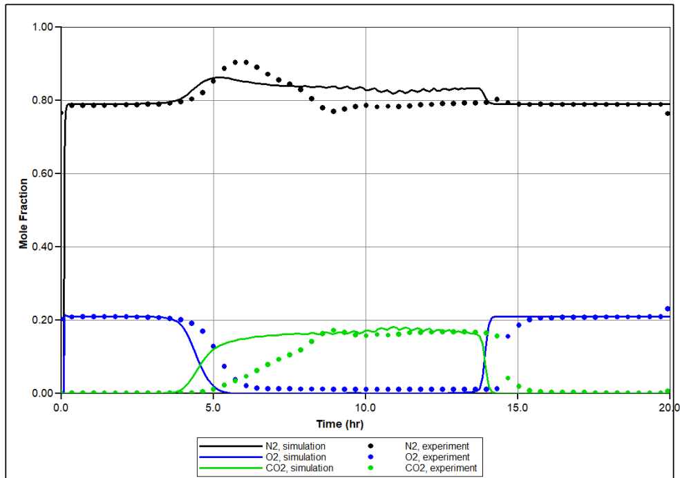
Figure 3.8 Comparison of the results for experiment and simulation for RTO test for bitumen: mole fraction of Nitrogen, Oxygen and Carbon Dioxide
