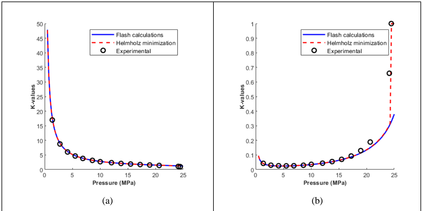
Figure 4.12 K-values at different pressures for the methane—n-heptane binary mixture at T = 344.3 K
