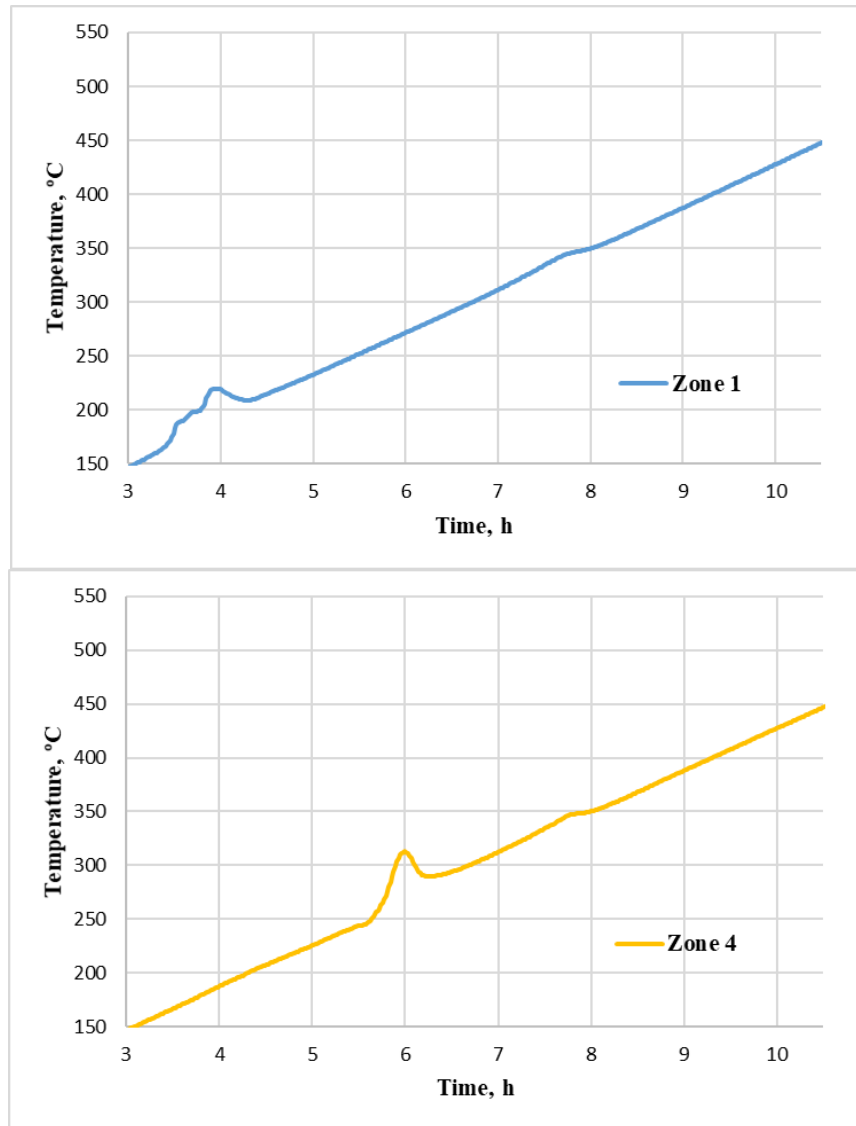
Figure 3.10 Zoom in temperature profiles for Zone 1 (above) and Zone 4 (below) in RTO test for carbonate oil field
