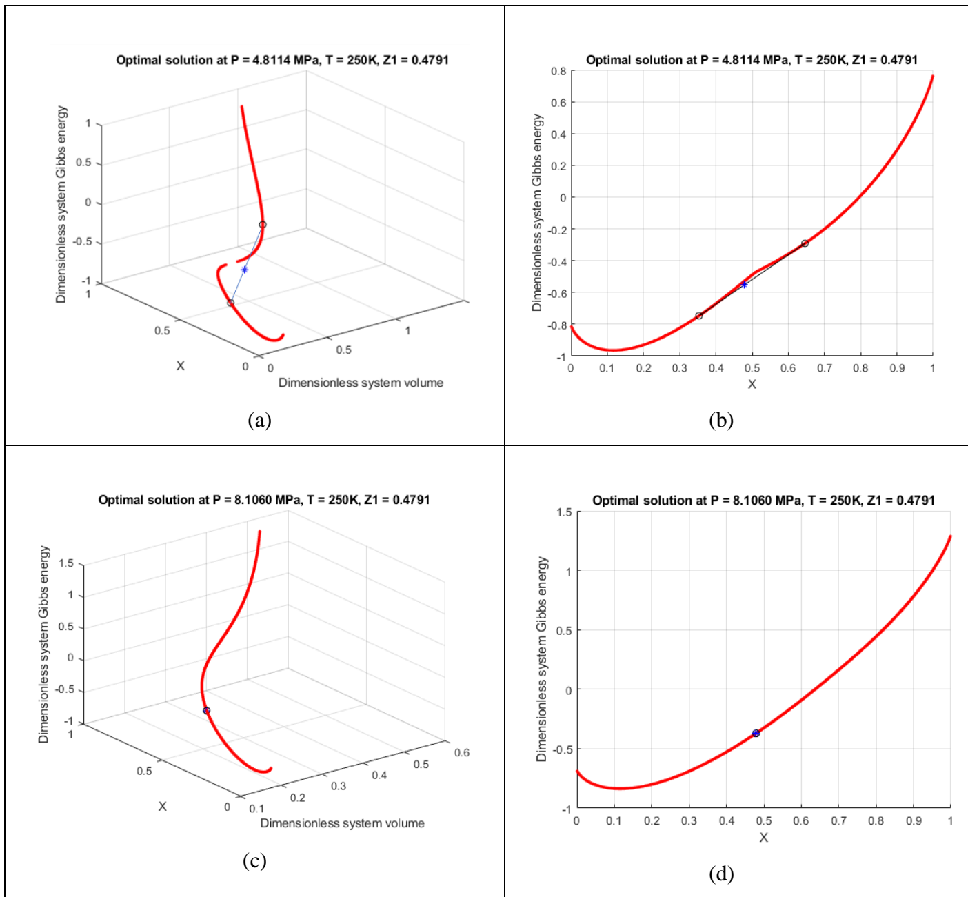
Figure 4.5. Visualization of the dimensionless system Gibbs energy in discrete compositional space for binary system Methane-Ethane under different initial conditions (blue star), and corresponding optimal solution (black circles). a,b) Initial conditions correspond to the two-phase region: P = 4.8114 MPa, T = 250 K, Z_1 = 0.4791 ; c,d) Initial conditions correspond to the critical region: P = 8.1060 MPa, T = 250 K, Z_1 = 0.4791 .
