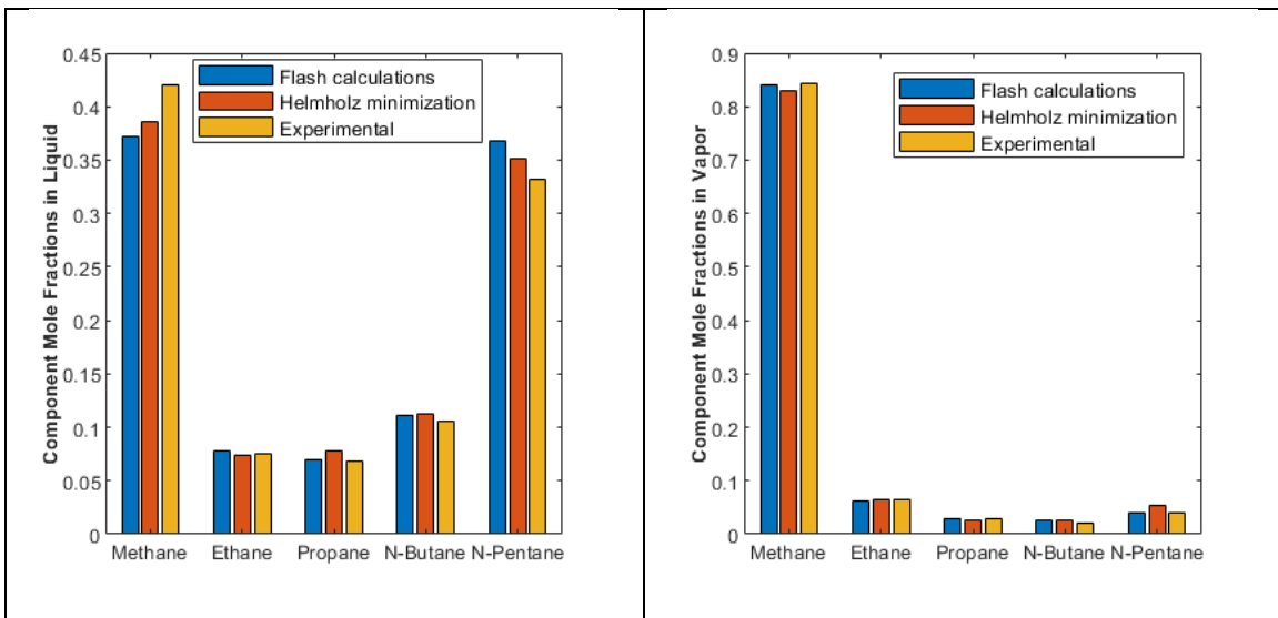
Figure 4.16 Phase compositions of the quinary mixture at P = 9.867 MPa and T = 311 K
