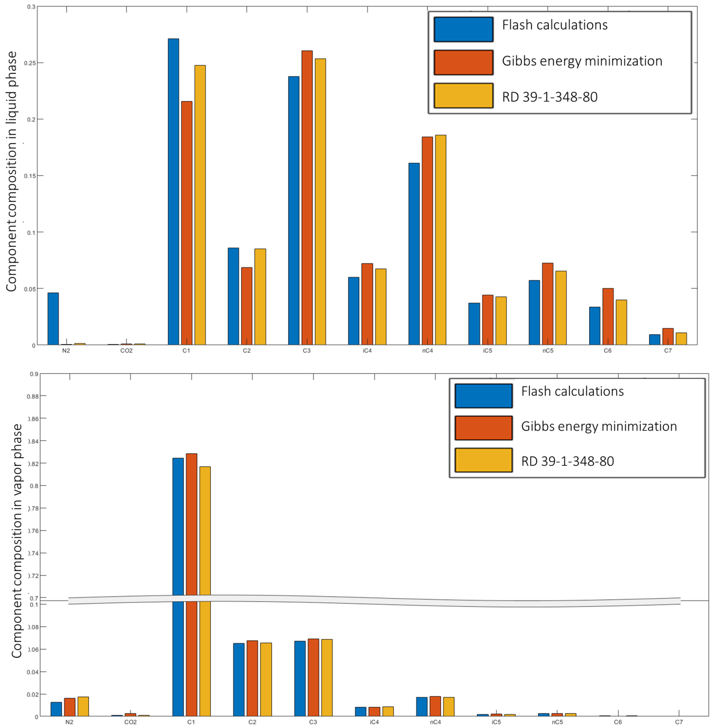
Figure 4.18 Phase compositions of the 11-component mixture: concentration of nitrogen, carbon dioxide, methane, ethane, propane, i-butane, n-butane, i-pentane, n-pentane, hexane and heptane in a) liquid and b) vapor phases in case of flash calculations (blue), Gibbs energy minimization algorithm (red) and experiment (orange)
