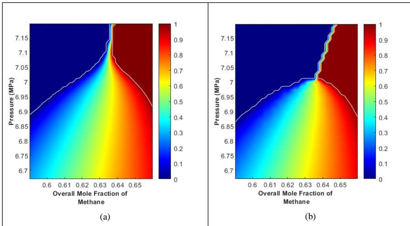
Figure 4.8 Zoomed fragment of the pressure-composition phase diagram for the methane—ethane binary mixture at T = 250\text{K} as a result of a) flash calculations and b) Gibbs minimization algorithm
