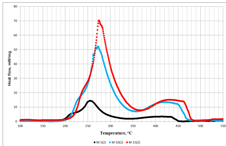
Figure 3.16 Temperature dependence of the heat flow for maltenes fraction of the original oil as a result of PDSC test (black - 5 °C/min, blue – 10 °C/min, red – 15 °C/min)
