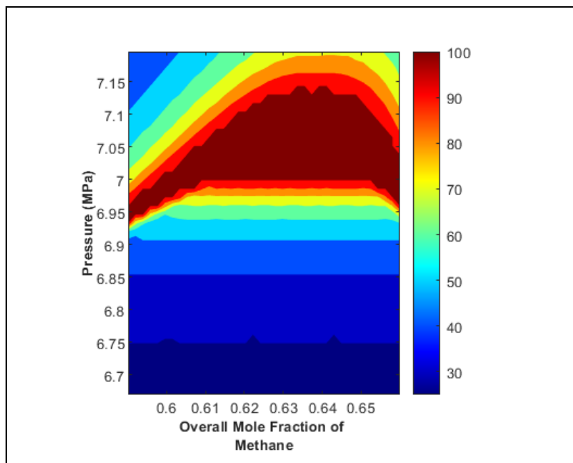
Figure 4.9 The actual number of iterations used in flash calculations (methane—ethane binary mixture)
