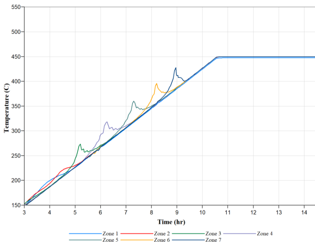
Figure 3.14 Zoom in simulated temperature profiles for the traditional reaction model for carbonate oil field
