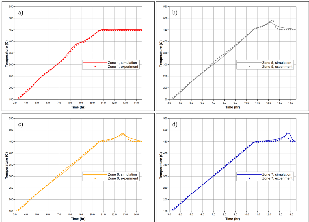
Figure 3.7 Comparison of numerical and experimental results for RTO test for bitumen: temperature profiles for a) 1 Zone; b) 5 Zone; c) 6 Zone and d) 7 Zones of the reactor
