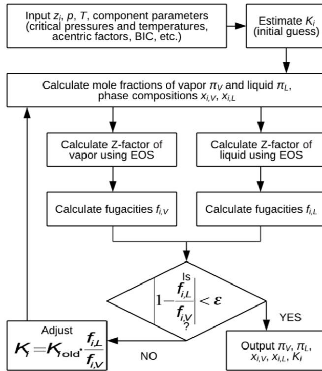
Figure 4.1 Flowchart of a) Helmholtz, b) Gibbs energy minimization algorithms and c) flash calculations (vapor-liquid equilibrium case)
