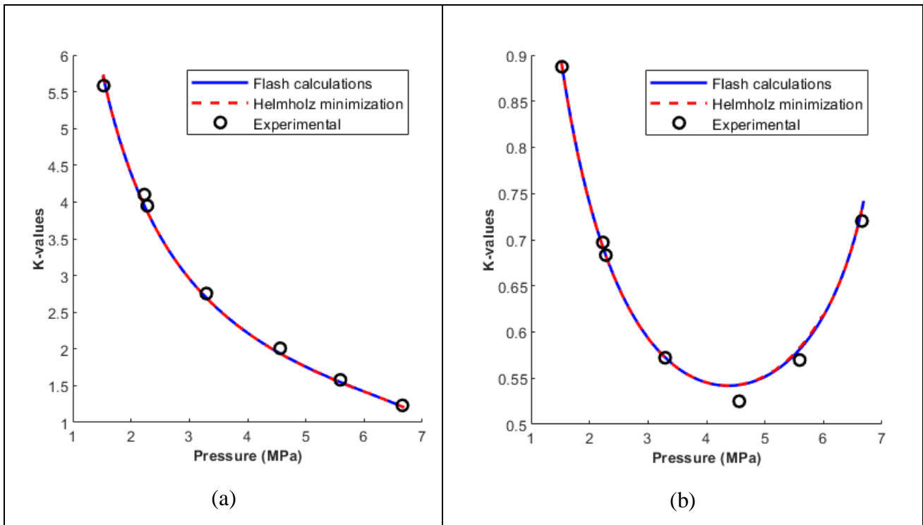
Figure 4.10-values at different pressures for the methane—ethane binary mixture at T = 250K
