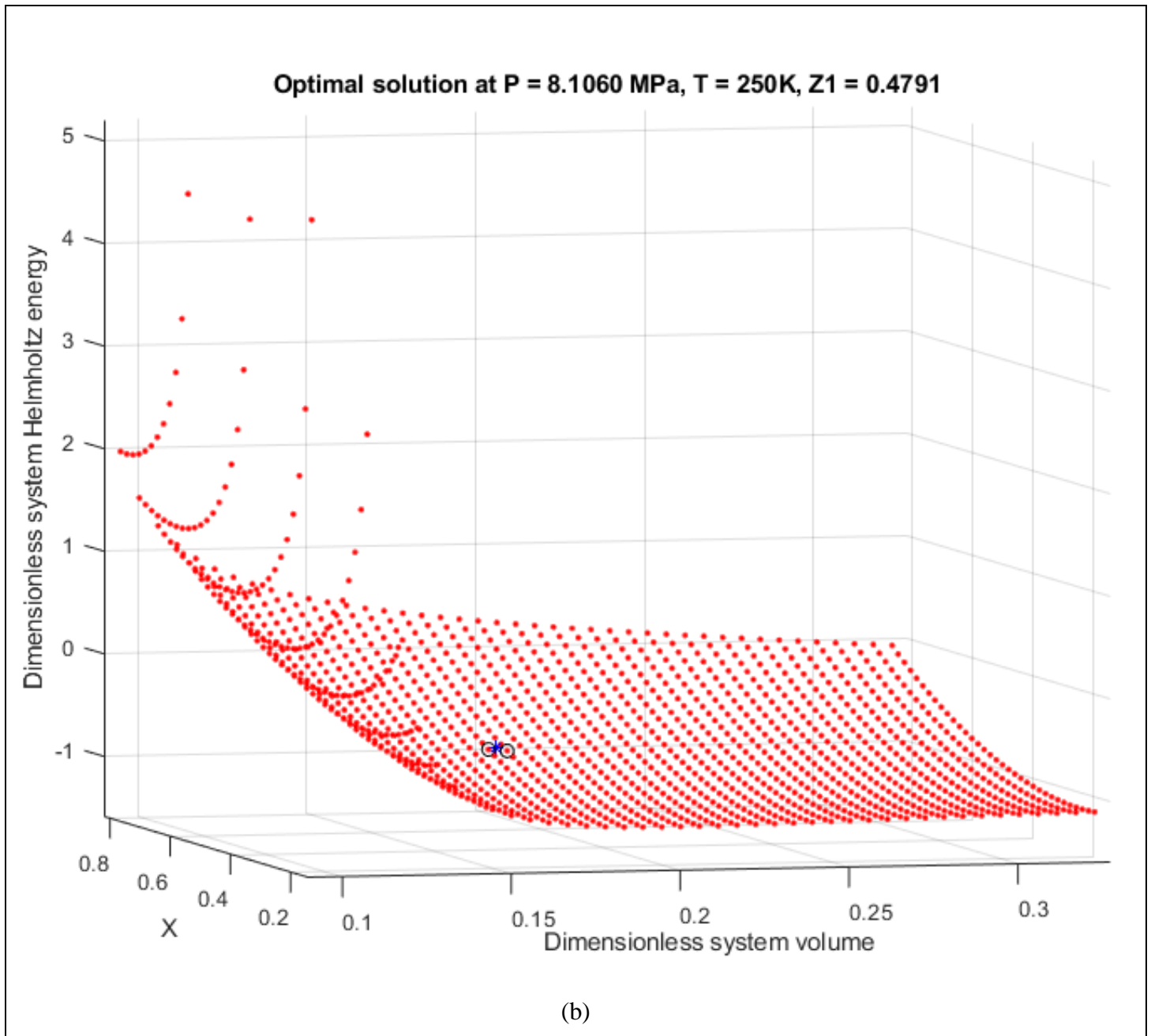
Figure 4.3. Visualization of dimensionless system Helmholtz energy in discrete volume and compositional space for binary system Methane-Ethane under different initial conditions (blue star), and corresponding optimal solution (black circles). a) Initial conditions correspond to the two-phase region: P = 4.8114 MPa, T = 250 K, Z_1 = 0.4791 ; b) Initial conditions correspond to the critical region: P = 8.1060 MPa, T = 250 K, Z_1 = 0.4791 .
