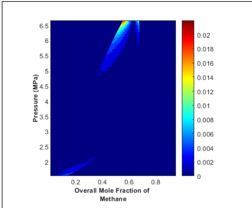
Figure 4.7 The modulus of the difference in molar fractions of the vapor phase calculated by flash calculations and the proposed Gibbs energy minimization technique (methane—ethane binary mixture)
