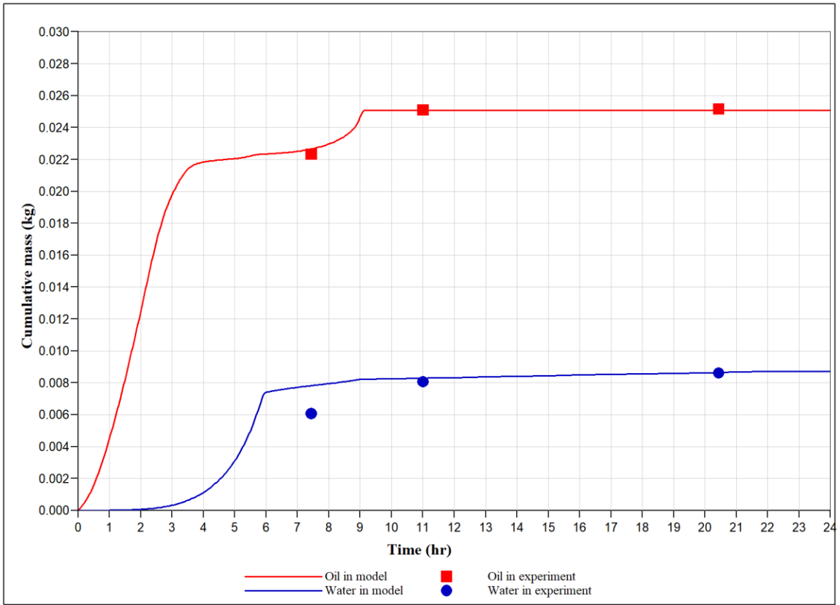
Figure 3.23 Comparison of the results for experiment and simulation for RTO test for carbonate oil example: cumulative oil mass and cumulative water mass (modified reaction scheme)
