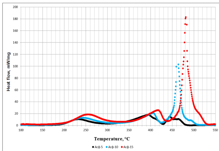
Figure 3.17 Temperature dependence of the heat flow for asphaltenes fraction of the original as a result of PDSC test (black - 5 °C/min, blue – 10 °C/min, red – 15 °C/min)
