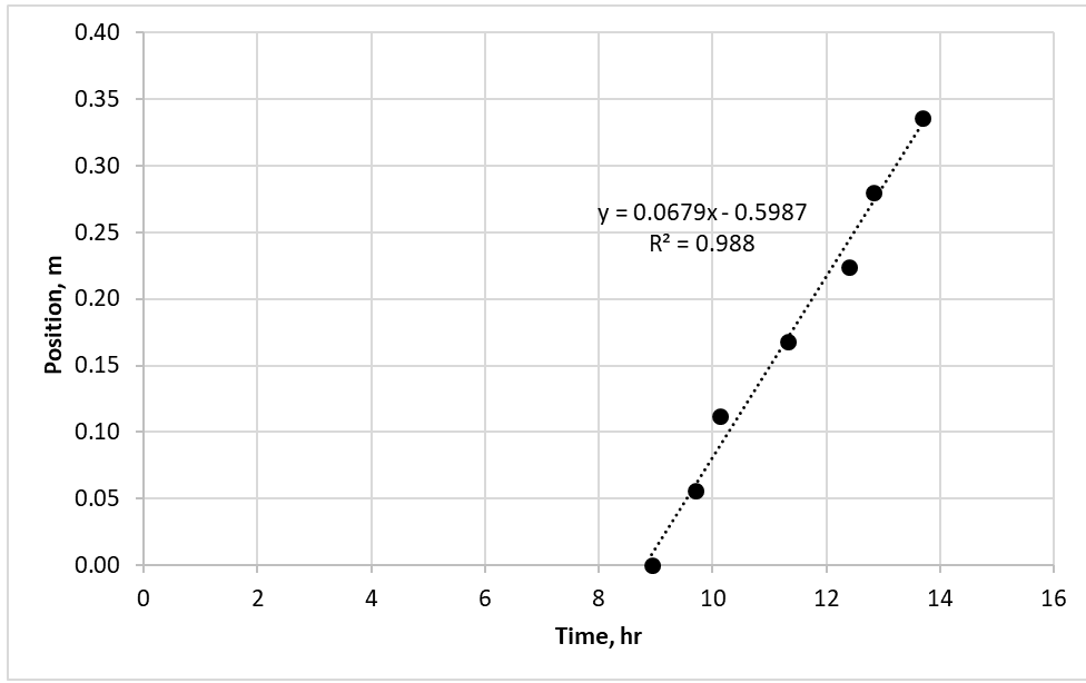
Figure 3.3 Combustion front propagation in HTR through zones 4-7 in RTO test for bitumen
