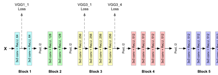
Fig. 6. Perceptual loss computation with pretrained VGG-19 network.
