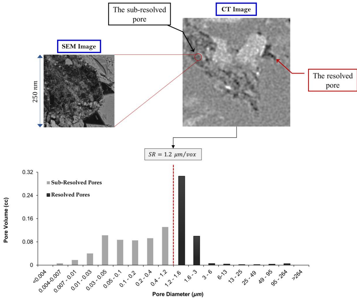
Figure 7: Comparing the results of PSD and the spatial resolution of \mu xCT images
