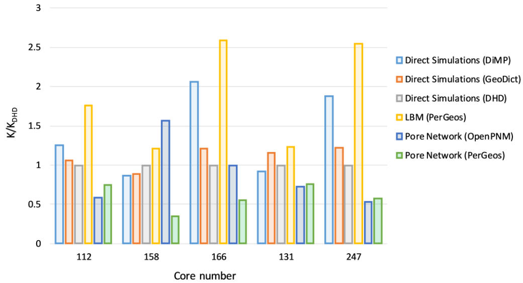
Figure 11: The results of permeability computations based on the variety of methods
