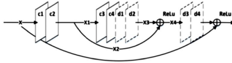
Figure 9: The schematic of the implemented RED-Net
