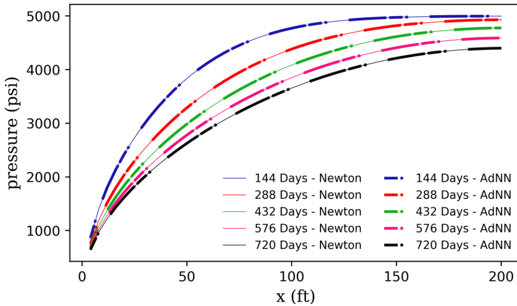
Figure 4: The results of using AdNN versus results of applying Newton’s method
