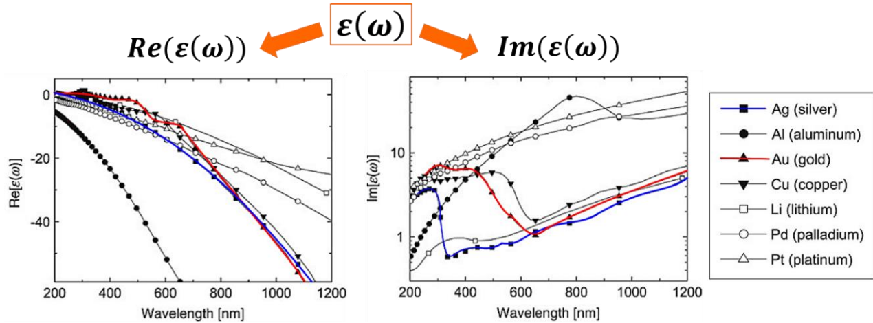
Figure 3-6. Real and imaginary parts of the dielectric function for different metals. Reproduced with permission from Le Ru et al. [159] Copyright © 2009 Elsevier B.V.
