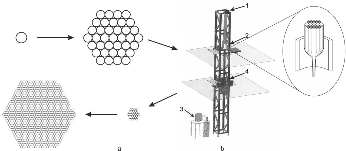
Figure 2-4. Schematic representation of the MOW manufacturing process (a) and MOW drafting unit (b): (1) billet feeding mechanism into the furnace; (2) furnace; (3) computer control; (4) drafting chain mechanism. Adapted from [29]
